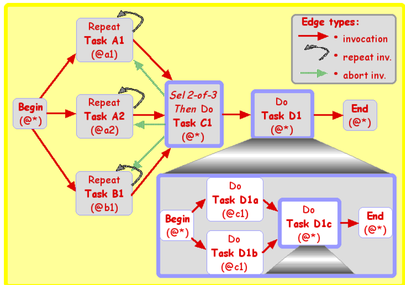
Figure 1: A tree and a graph view of taskflow hierarchy, represented as blackboxes and whiteboxes.
