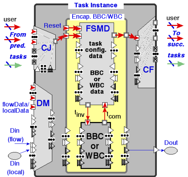
Figure 2: Layered primitives of the task model.
