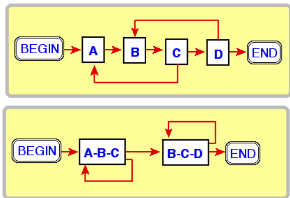
Figure 6: Restructuring a pattern of arbitrary cycles to a pattern with structured cycles.
